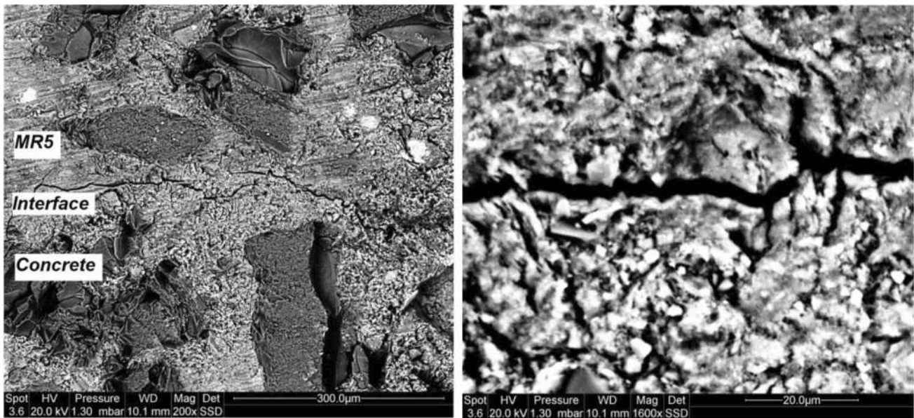
Fig. 16 SEM images of mixed mortar–concrete sample MR5 showing cracks at the interface (magnified views at 200× (left) and 1600× (right))
