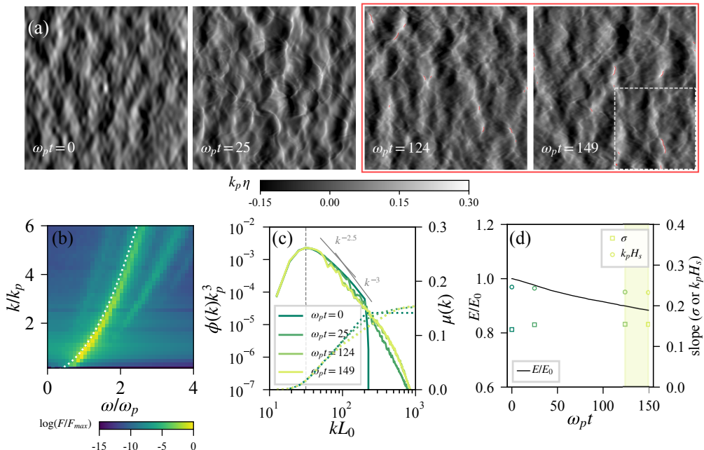
FIGURE 3. (a) Snapshots of the wave field development for the case of rms slope \sigma = 0.153 . Breaking statistics are collected between \omega_p t = 124 and \omega_p t = 149 (indicated by the red box). (b) The wave energy spectrum on the frequency-wavenumber plane. The dotted white line is the linear dispersion relation of surface gravity waves k = \omega^2/g . (c) Time evolution of the omni-directional wave spectrum \phi(k) , corresponding to the snapshots in (a). (d) Energy and \sigma slope evolution of the wave field. Black line: evolution of wave energy (as the sum of potential and kinetic energy integrated over the whole field). Squares: the rms slope \sigma of the four snapshots shown in (a); circles: the effective slope k_p H_s of the four snapshots shown in (a). The breaking statistics are collected during the shaded time interval.
