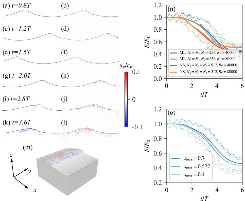
FIGURE 2. (a)(c)(e)(g)(i)(k): Snapshots of the wave profile and span-wise velocity u_y on the y = 0 central plane slice at time t = (0.8, 1.2, 1.6, 2.0, 2.8, 3.6) T . of the multi-layer solver ( 256 \times 256 \times 15 grid); (b)(d)(f)(h)(j)(l): two-phase Navier-Stokes solver ( 256 \times 256 \times 256 grid) at the same times. (m): 3D rendering of the single breaking wave case in the multi-layer solver at t = 3.6T . Initial wave steepness ak = 0.35 , and Reynolds numbers Re \equiv \sqrt{g\lambda^3}/\nu = 40000 where \lambda is the wavelength. (n): the energy dissipation of the two solvers compared. Dashed line: two times kinetic energy; dotted line: two times potential energy; solid line: total energy. Initial wave steepness ak = 0.35 . (o): the energy dissipation is not sensitive to the specific value of the gradient limiter threshold s_{max} . Initial wave steepness ak = 0.35 , Re = 40000 .
