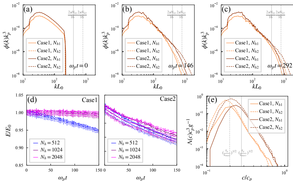
FIGURE 9. Convergence between horizontal grid point N_h = 1024 and 2048 . (a)(b)(c): wave energy spectra at \omega_p t = 0, 146, 292 respectively. The gray vertical lines indicate k_{\max}L_0 for N_h = 1024 and 2048 respectively. (d): energy evolution for Case1 and Case2 with varying horizontal grid points N_h . Solid lines: total energy; dashed lines: two times kinetic energy; dotted lines: two times potential energy. (e) Breaking distribution for Case1 and Case2 with varying horizontal grid points N_h . The gray vertical lines indicate the phase speed k_{\max} for N_h = 1024 and 2048 respectively.
