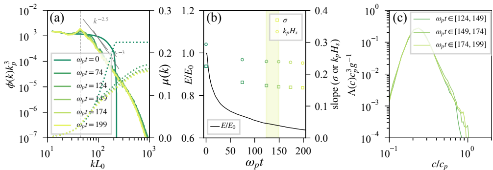
FIGURE 7. (a)(b) Same as figure 3 but with the initially Gaussian spectra cases. A quasi steady state spectrum is obtained after O(100\omega_p t) , with a k^{-3} shape. (c) The \Lambda(c) distribution computed during different time windows in the quasi steady regime.
