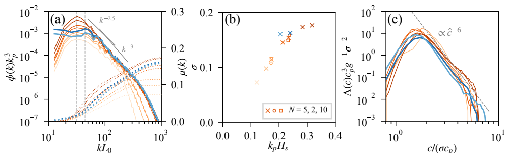
FIGURE 8. Same as figure 5 comparing the initially Gaussian spectra cases and the wind-wave initial spectra. Once a quasi-steady state is reached (due to breaking and loss of excess energy), the wave spectra and breaking distribution are comparable.
