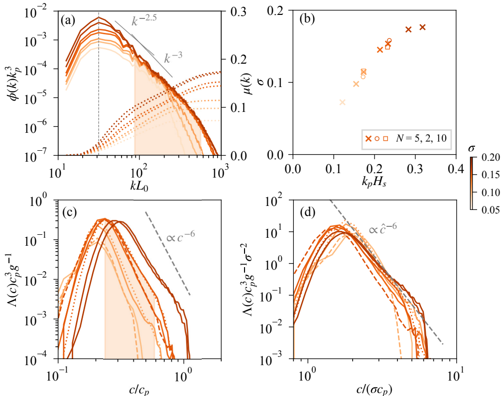
FIGURE 5. Wave energy spectra of different steepness and their \Lambda(c) distribution. The colours correspond to different \sigma slopes according to the colour bar. (a) The wave energy spectra during the breaking statistics collection time interval in non-dimensional form; the vertical gray line is k_p L_0 = 10\pi . Darker colour indicates larger global slope k_p H_s (see (b) for the values). (b) The correlation of rms slopes \sigma and the global slopes k_p H_s in the simulated cases. Crosses: N = 5 ; circles: N = 2 ; squares: N = 10 . (c) The non-dimensional breaking distribution \Lambda(c) normalised by c_p and g . Solid lines: directional spreading parameter N = 5 ; dashed lines: N = 2 ; dotted lines: N = 10 . (d) Proposed scaling for the \Lambda(c) distribution using \sigma and c_p . The pre-factor of the dotted line is 800.
