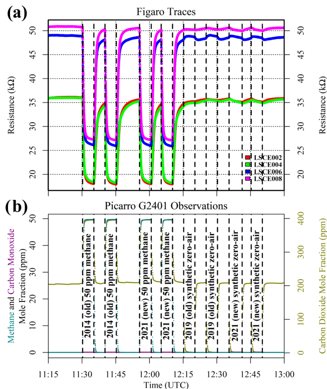
Figure 4. (a) Measured resistance for four Figaro sensors in System B (coloured dots; see legend) under exposure to two sources of 50 ppm methane mole fraction and two sources of synthetic zero air (all compared to gas from a zero-air generator). (b) Corresponding Picarro G2401 mole fraction observations, with annotations indicating the synthetic cylinder type. Areas not annotated correspond to gas from the zero-air generator. Methane (dark cyan) and carbon monoxide (dark magenta) mole fraction measurements are plotted on the left-hand axis. Carbon dioxide (dark yellow) mole fraction measurements are plotted on the right-hand axis.
