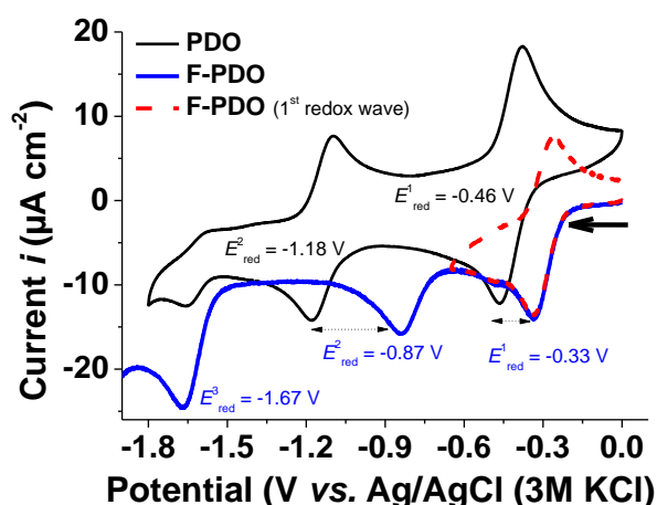
Figure 4. Comparison of the CV spectra of F-PDO (blue line, 1 st cycle) and PDO (black line). Solvent: DMSO; I = 0.1 M n\text{-Bu}_4\text{NPF}_6 ; v = 200 \text{mV s}^{-1} ; T = 23(1) °C. Reference electrode = \text{KCl}(3\text{ M})/\text{Ag}/\text{AgCl} ; working electrode = glassy carbon disk of 0.07\text{ cm}^2 area; auxiliary electrode = Pt wire. Starting potential = 0 V. IUPAC convention used to report the CV data. The solid arrow indicates the direction of scan.
