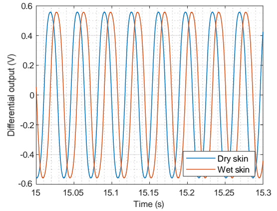
Fig. 8. Transient simulation
