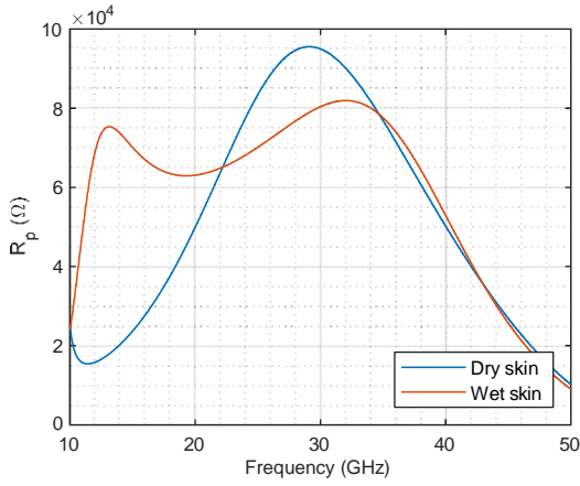
Fig. 4. Real part of the sensor impedance with dry and wet skin
