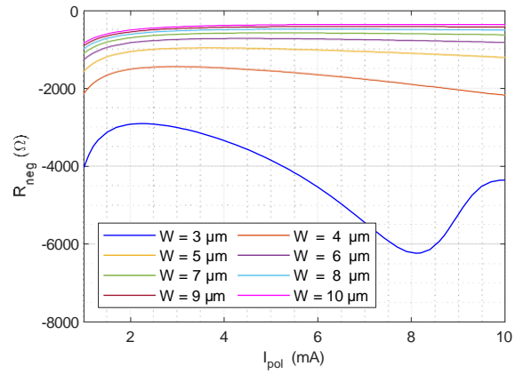
Fig. 5. Negative impedance variation
