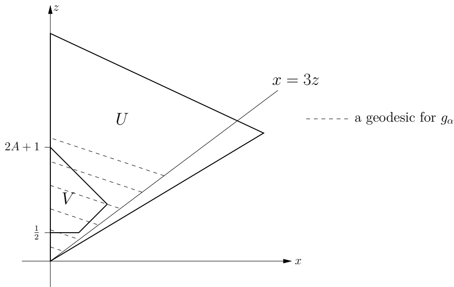
FIGURE 1. The geodesics of g_\alpha
