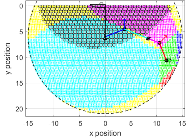
Figure 5: Areas for an umbilical with two sliding elements and an anchor. Green: A0. Blue: A11. Cyan: A12. Red: A21. Magenta: A22. Yellow: areas D. Black: area F where the umbilical cannot be stretched. Blue arrow : force \vec{F}_1 . Red arrow: force \vec{F}_2 .
