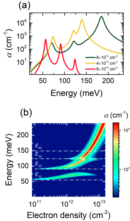
Figure 2. (a) Absorption coefficient for a 8 nm-thick 30% Mg ZnO/ZnMgO QW with various electron concentrations at RT. (b) Color map showing the absorption coefficient of said QW as a function of the 2D electron concentration. The energies of the bare 1 → 2, 2 → 3, 3 → 4, and 4 → 5 ISBTs are indicated.
