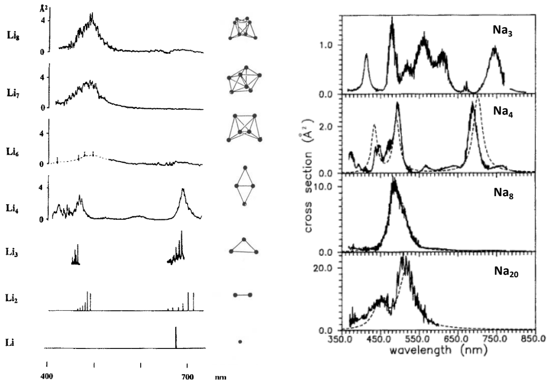
figure 3 : (left) Absorption spectra of Lin clusters n=1-8 . The results for n \leq 3 were recorded by means of resonant two-photon ionization, while the results for n > 3 were obtained by means of depletion spectroscopy. The corresponding geometries result from the comparison of the spectra with CI ab initio calculations. Reproduced by permission from ref.[33], Copyright © by R. Oldenbourg Verlag, München 1996. (right) Absorption spectra of Nan clusters n=3, 4, 8 and n=20 , obtained by depletion spectroscopy. Reproduced by permission from ref [34] Copyright © by Springer-Verlag 1991.
