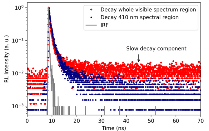
Figure 5. Time decay of luminescence excited by soft X-ray (sample P1). The whole visible spectral region measured (red), and with a filter centered at 410 nm (dark blue). Instrument response function (IRF) is also plotted (grey).
