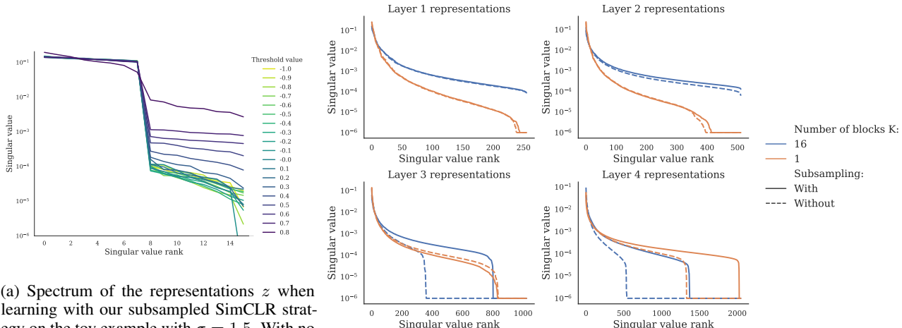
(b) Spectrum of the intermediate representations (h_i^k)_i after each of the 4 ResNet layers on CIFAR-10; with models decoupled ( K = 16 ) or not ( K = 1 ) and trained with our without subsampling. With no subsampling, the spectra exhibit a fast decay at later layers, indicating a dimensionality collapse, while our subsampling results in a much higher features dimensionality even for K = 1 .
