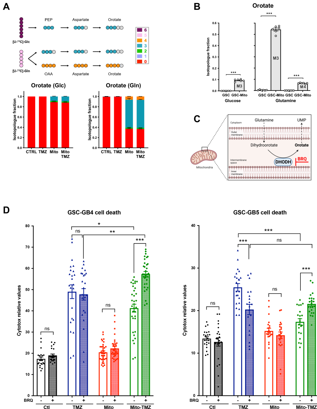
FIGURE 6 MSC mitochondria induce a higher orotate turnover in GSCs which supports resistance to TMZ. A and B , [ 13 C]-glucose and [ 13 C]-glutamine orotate isotope profiling in GSCs with and/or without MSC mitochondria and treated or not with TMZ (48 hours; n = 3). Mean + SEM. Statistical analysis by Student t test. ***, P < 0.001. C , Schematic of BRQ inhibition of DHODH-dependent orotate production (BioRender). D , Effect of BRQ (100 nmol/L) on the survival of GSCs (GB4 and GB5, from 2 donors) to TMZ treatment (50 μmol/L) following acquisition of MSC mitochondria (3 MSC donors for each GSC). Two-way ANOVA, *, P < 0.05; **, P < 0.01; ***, P < 0.001; n = 4, each dot represents a culture well.
