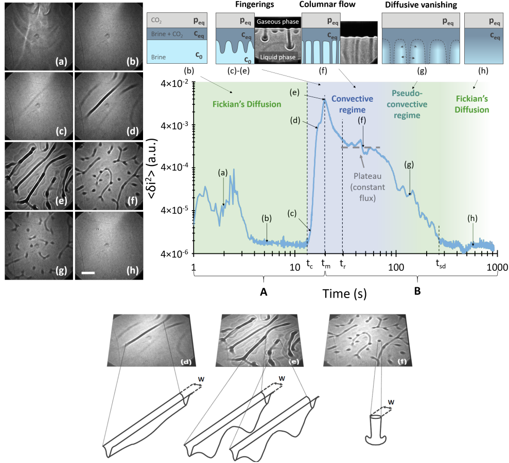
FIG. 2: 3D spatio-temporal evolution of the convective dissolution process for \text{CO}_2 dissolved in pure water for a pressure increase from 0.1 to 2.1 MPa. Top-left panel: Shadowgraph images taken at different times of the process. Top-right panel: Time evolution of the variance \langle \delta i^2 \rangle of shadowgraph image differences. The top inserts show schematically the boundary layer and the patterns with representative images obtained from transversal observation. (a) The injection temporarily perturbs the contrast until the gaseous phase becomes stable and the contrast constant. (b) During this regime, \text{CO}_2 spreads diffusively into water, giving rise to an unstable growing boundary layer. (c) At t = t_c , the contrast rises and convective patterns suddenly appear. (d) After a short time, the first pattern reaches the maximum concentration C_{\text{eq}} of \text{CO}_2 and further patterns appear. (e) The image variance reaches a maximum at t_m . (f) The plateau characterizes a stationary condition where the boundary layer thickness and the convective flux are constant. Here, the convective flow is essentially made of plumes. (g) The convective flow gradually mixes \text{CO}_2 and water in the entire bulk, and patterns become less and less contrasted as they are dissipating diffusively. (h) Convection vanishes and the variance goes back to its initial level. The size bar in (h) corresponds to the water layer thickness h=2 mm. Bottom panel: Schematic representation of the convective patterns. (left)
