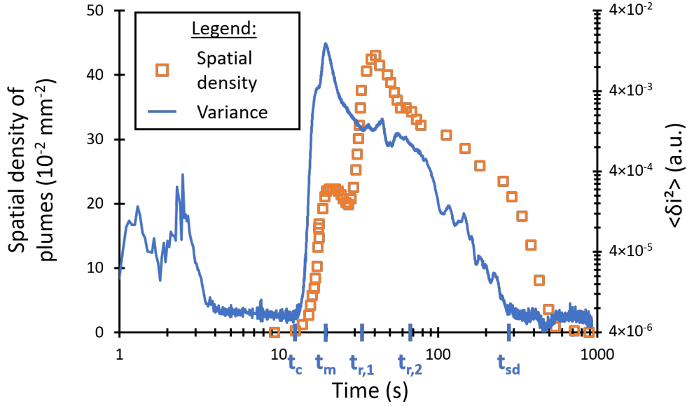
FIG. 3: Plume density measured from the shadowgraph images for an injection from 0.1 to 2.1 MPa (orange square symbols) plotted against optical contrast as in Fig. 2 (blue continuous line). After t_c , plumes appear within the sheets and the plume density rises. The latter reaches a first maximum around t_m , decreases and rapidly increases again after t_r due to the appearance of isolated plumes. Then, the plume density decreases and vanishes after t_{sd} that corresponds to the end of the convective regime. The typical timescales defined in figure 2 have been reproduced here on the axis of time.
