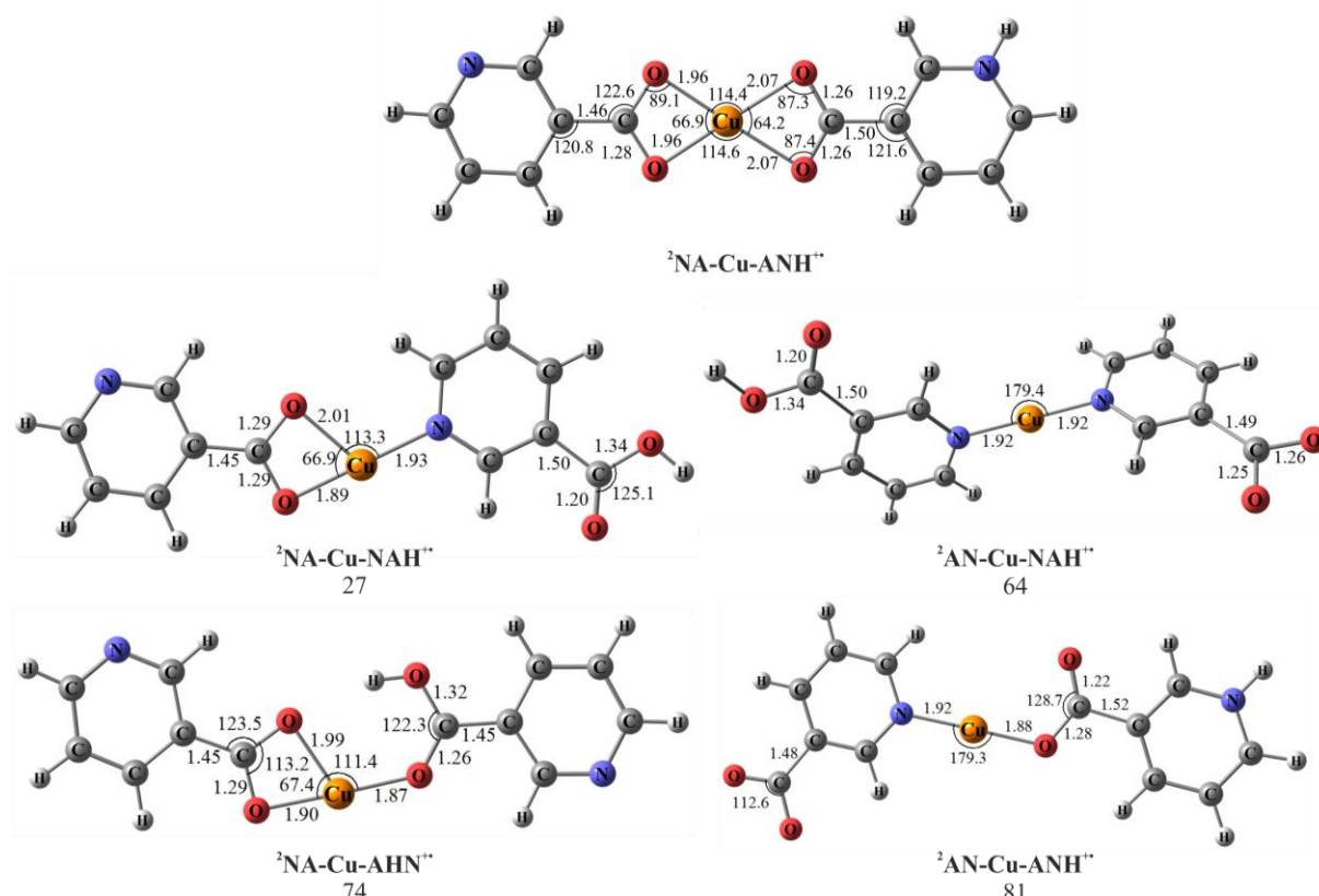
Figure S2. Geometry optimized structures and relative energies of the various [Cu + 2NAH – H] + complexes considered. Relative energies are in kJ/mol. bond lengths in Å and angles in degrees.
