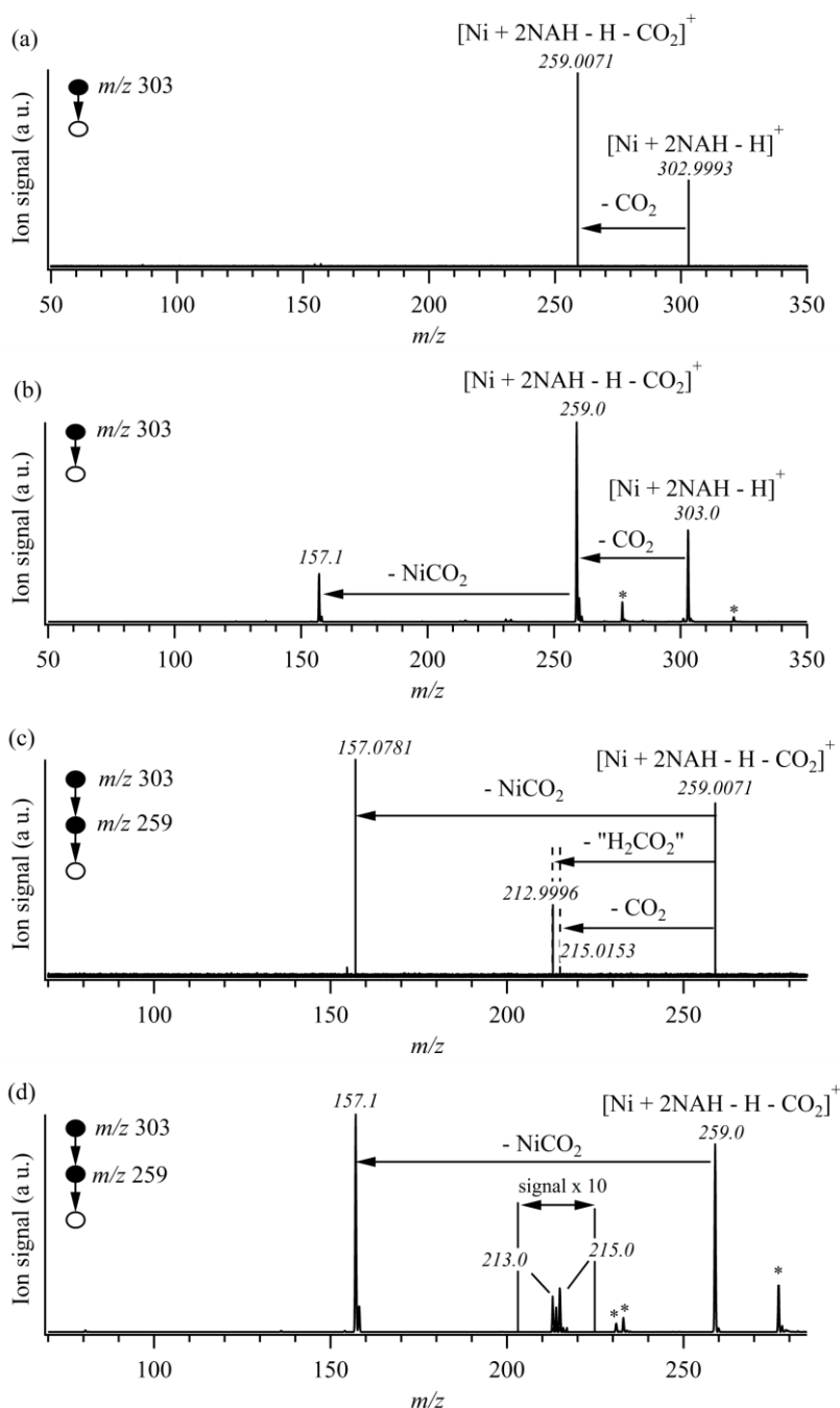
Figure 4. MS 2 - (a) SORI-CID (FT-ICR) and (b) CID (ion trap) spectra of [\text{Ni} + 2\text{NAH} - \text{H}]^+ ( m/z 303) and MS 3 (c) SORI-CID and (d) CID spectra of [\text{Ni} + 2\text{NAH} - \text{H} - \text{CO}_2]^+ ( m/z 259). In spectra (b) and (d), some ions have captured a water molecule due to the presence of water in the trap. These water adducts are indicated by an asterisk.
