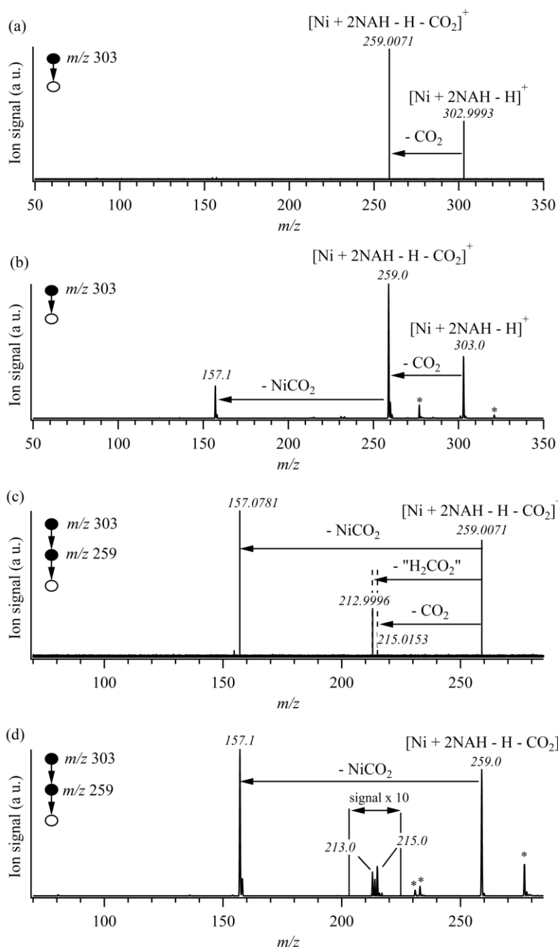
Figure 4. MS 2 - (a) SORI-CID (FT-ICR) and (b) CID (ion trap) spectra of [Ni + 2NAH - H] + ( m/z 303) and MS 3 (c) SORI-CID and (d) CID spectra of [Ni + 2NAH - H - CO 2 ] + ( m/z 259). In spectra (b) and (d), some ions have captured a water molecule due to the presence of water in the trap. These water adducts are indicated by an asterisk.
