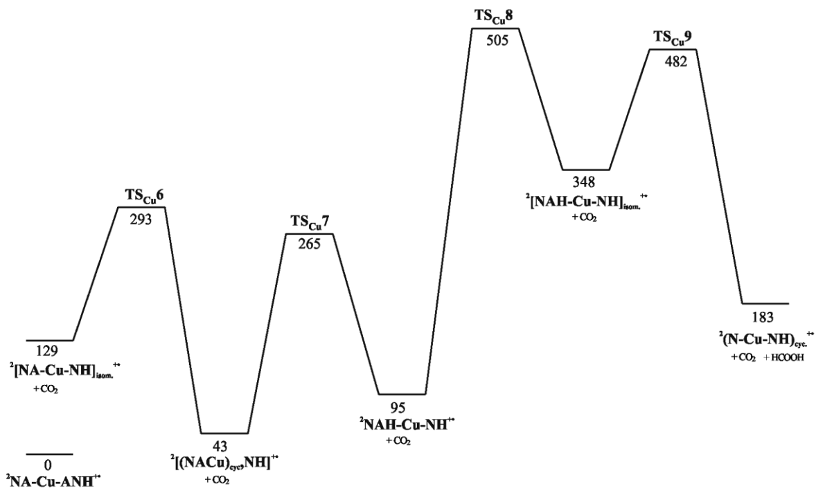
Figure S5. Potential energy diagram for HOCOH loss of NA-Cu-NH ++ ion (relative energies in kJ/mol).
