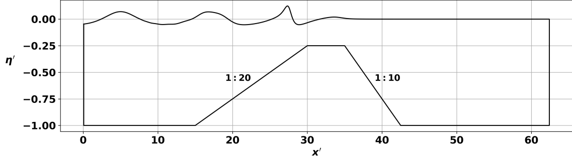
Figure 8: Computational domain used in 2D-NWT simulations of quasi-regular wave propagating over a submerged bar. An absorbing beach of length l'_{AB} is specified at the far-end of the domain, starting at x' = 42.5 .
