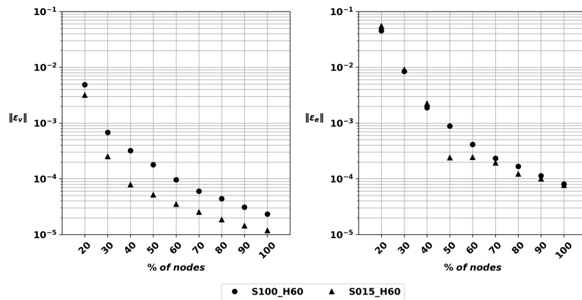
Figure B.3: Convergence analysis of the the maximum errors of mass ( \|\epsilon_v\| , left) and energy ( \|\epsilon_e\| , right) of the solitary wave at t_b as a function of the BEM grid discretization for the two beach slope configurations.
