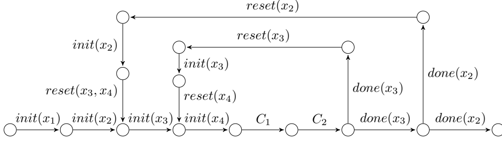
Figure 7: Schema of construction for TQBF instance \exists x_1 \forall x_2 \forall x_3 \exists x_4 ((x_1 \vee \overline{x_4}) \wedge (\overline{x_2} \vee \overline{x_3} \vee x_4)) .
