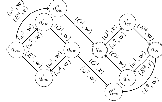
Figure 4: The 2-LaMA \llbracket A_h \rrbracket_\zeta , encoding of the HRA A_h from Fig. 3.
