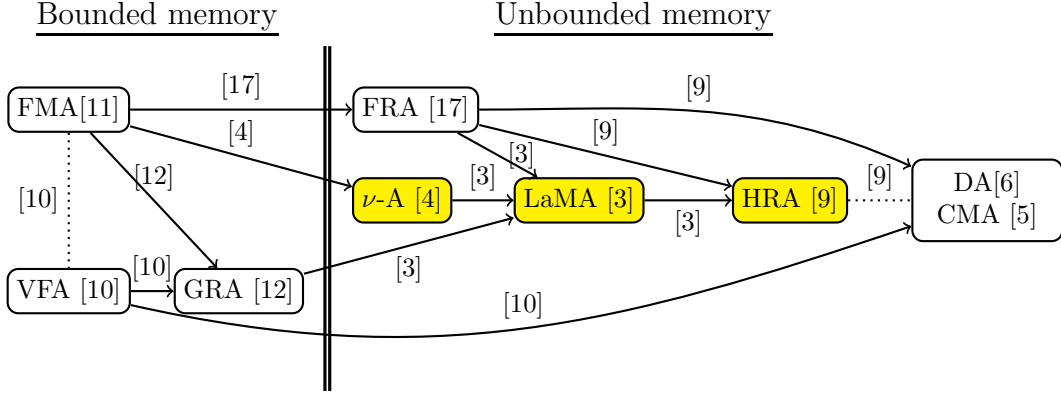
Figure 1: A classification of memory automata from [3]. Arrows represent strict language inclusion, while dotted lines denote language incomparability. Formalisms studied here are in yellow.
