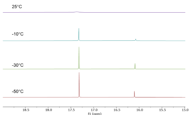
Figure 7. Variable temperature ^1\text{H} NMR spectra of complex 7b in the region 19.0-15.0 ppm ( \text{THF-d}_8 , 600 MHz).
