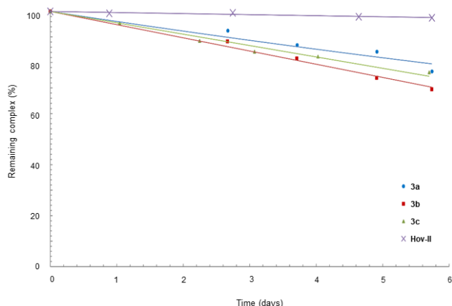
Figure 3. Stability tests of Hoveyda-type complexes 3a-c and Hov-II in toluene- d_8 at 50 °C under argon. Monitored by ^1\text{H} NMR spectroscopy using 1,3,5-trimethoxybenzene as internal standard. Lines placed as visual aids.
