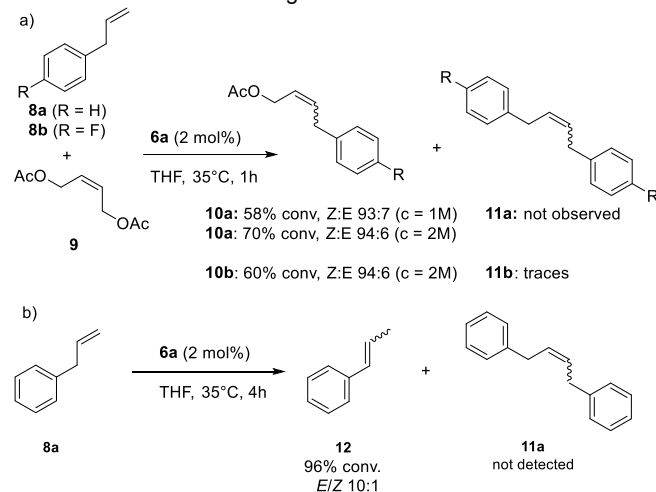
Scheme 4. a) Cross-metathesis of allylarenes 8a-b with cis -1,2-diacetoxy-2-butene 9 catalyzed by 6a . b) Isomerization of allylbenzene 8a upon treatment with 6a . Conversions were determined by GC analysis against a calibrated internal standard (tetradecane).
