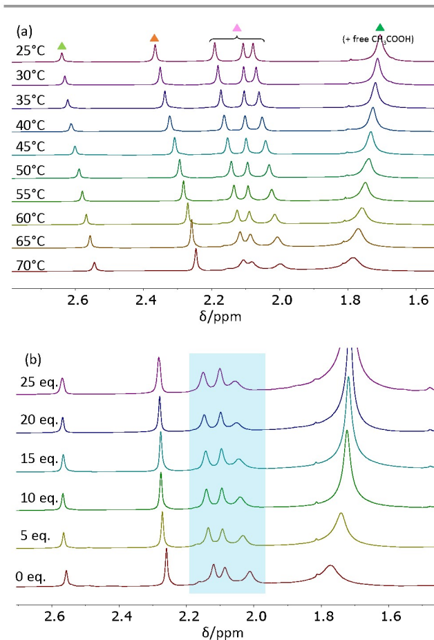
Figure 6. ^1\text{H} NMR spectra (400 MHz) of [\text{Zr}_6\text{O}_4(\text{OH})_4(\text{O}_2\text{CMe})_{12}]_2 (8.0 mg) in C_6D_6 (0.8 mL) in the acetate Me resonance region: (a) at variable-temperature between 25 and 70^\circ\text{C} ; (b) with different amounts of added free acetic acid at 65^\circ\text{C} ( 1.14\ \mu\text{L} = 5 equivalents of acetic acid per Zr_{12} unit).
