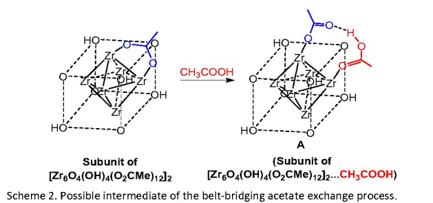
Scheme 2. Possible intermediate of the belt-bridging acetate exchange process.
