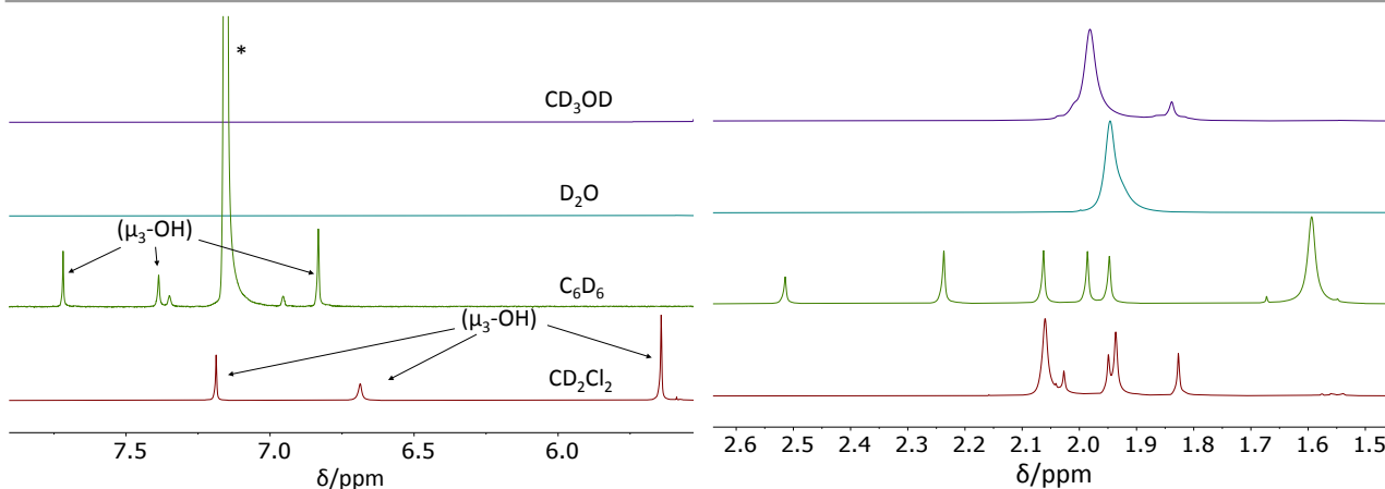
Figure 2. Room temperature ^1\text{H} NMR spectra (400 MHz) obtained for solutions of [\text{Zr}_6\text{O}_4(\text{OH})_4(\text{O}_2\text{CMe})_{12}]_2 in various solvents in the OH and Me regions. The starred resonance is due to the residual solvent \text{C}_6\text{D}_5\text{H} in \text{C}_6\text{D}_6 , with its spinning side bands.
