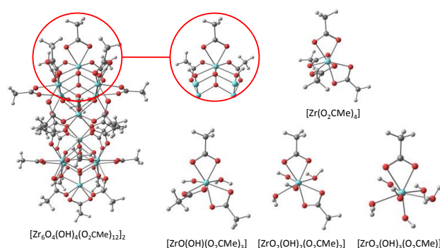
Figure 7. Geometries of the [\text{Zr}_6\text{O}_4(\text{OH})_4(\text{O}_2\text{CMe})_{12}]_2 molecule and of the mononuclear models used for the DFT calculation of the chelating acetate exchange.
