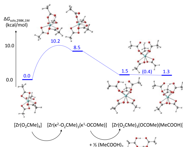
Figure 8. Gibbs energy profile (25 °C in dichloromethane, 1 M standard state) of the chelating acetate exchange in [Zr(O 2 CMe) 4 ].
