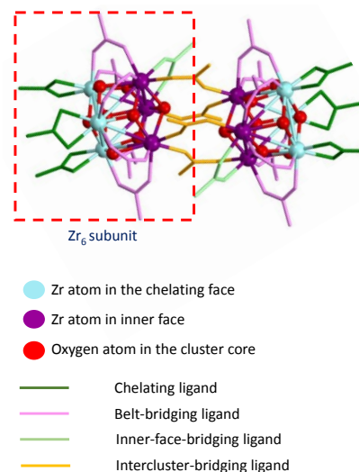
Figure 1. Schematic view of the [\text{Zr}_6\text{O}_4(\text{OH})_4(\text{O}_2\text{CMe})_{12}]_2 structure.
