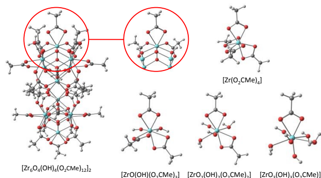
Figure 7. Geometries of the [Zr 6 O 4 (OH) 4 (O 2 CMe) 12 ] 2 molecule and of the mononuclear models used for the DFT calculation of the chelating acetate exchange.
