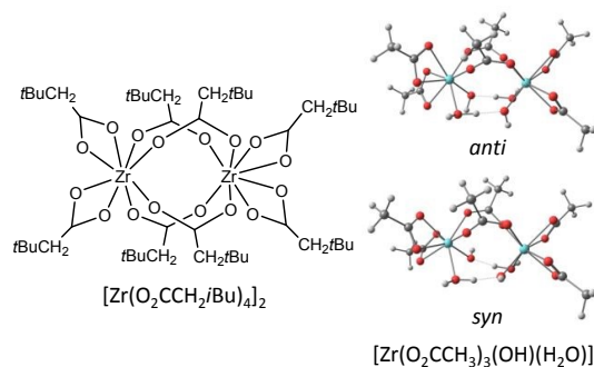
Figure 10. Geometries of the [\text{Zr}(\text{O}_2\text{CH}_2\text{tBu})_4]_2 molecule and of the [\text{Zr}(\text{O}_2\text{CMe})_3(\text{OH})(\text{H}_2\text{O})] models used for the DFT calculation of the comparative chelating and bridging acetate exchange.
