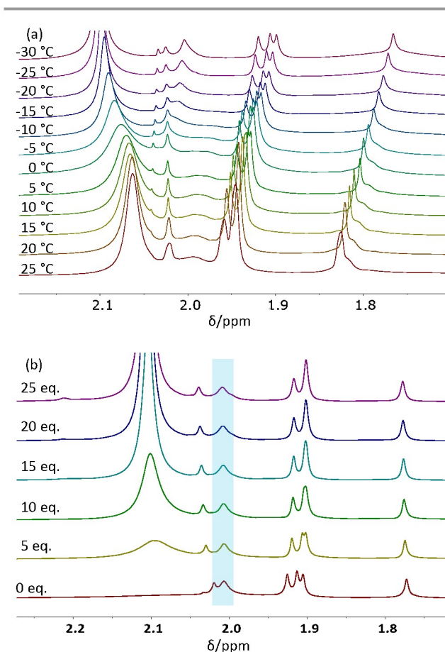
Figure 4. 1 H NMR spectra (600 MHz) of [Zr 6 O 4 (OH) 4 (O 2 CMe) 12 ] 2 (5.3 mg) in CD 2 Cl 2 (0.8 mL) in the acetate Me resonance region: (a) at variable-temperature between 25 and -30 °C; (b) with different amounts of added free acetic acid at -20 °C (1.14 \mu L = 5 equivalents of acetic acid per Zr 12 unit). Note that the batch used for the investigation Figure 4b is different and contains much less free acetic acid than that used for the variable-temperature investigation of Figure 4a.
