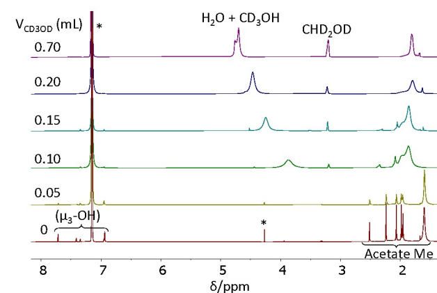
Figure 3. Room temperature 1 H NMR spectra (400 MHz) of [Zr 6 O 4 (OH) 4 (O 2 CMe) 12 ] 2 in a C 6 D 6 /CD 3 OD solvent mixture in the OH and Me regions. The solutions were obtained by subsequent additions of CD 3 OD to the initial solution of 8.8 mg of the cluster in 0.5 mL of C 6 D 6 . The starred resonances are due to the residual C 6 D 5 H in the solvent (with its spinning side-bands) and to co-crystallized CH 2 Cl 2 .
