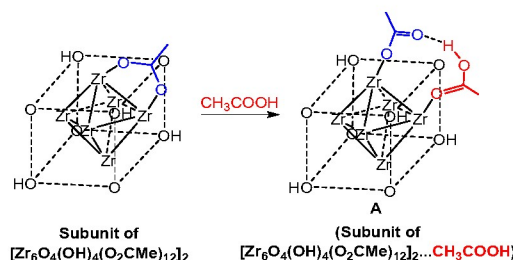
Scheme 2. Possible intermediate of the belt-bridging acetate exchange process.
