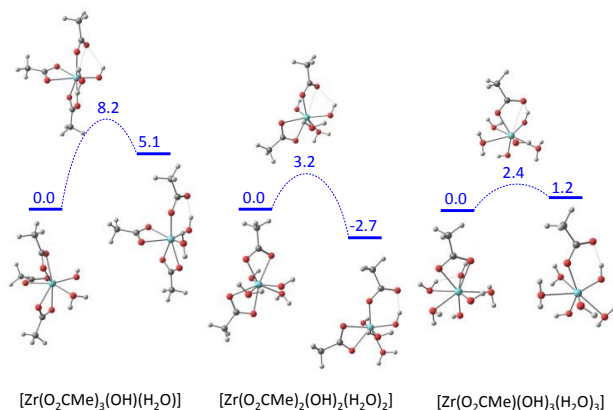
Figure 9. Gibbs energy profile (25 °C in dichloromethane, 1 M standard state) of the chelating acetate partial dissociation in [\text{Zr}(\text{OH})(\text{H}_2\text{O})(\text{O}_2\text{CMe})_3] , [\text{Zr}(\text{OH})_2(\text{H}_2\text{O})_2(\text{O}_2\text{CMe})_2] and [\text{Zr}(\text{OH})_3(\text{H}_2\text{O})_3(\text{O}_2\text{CMe})] .
