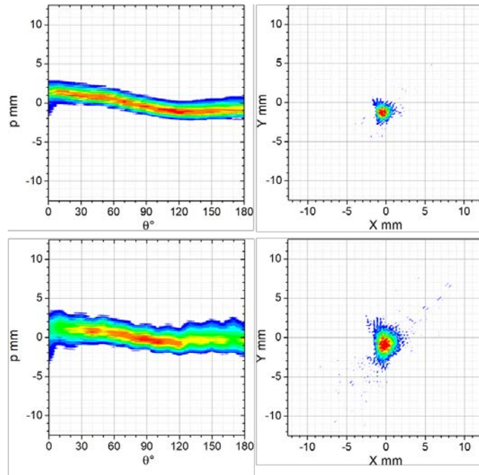
Figure 7: Effect of focalization. Left: sinogram, right: density. Top: good focalization (300V), bottom: bad focalization (350V)
