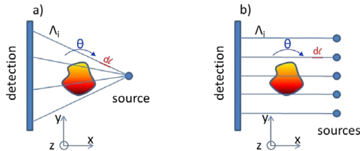
Figure 1: Principle of RX tomography a) with a point x ray source, b) parallel beams
