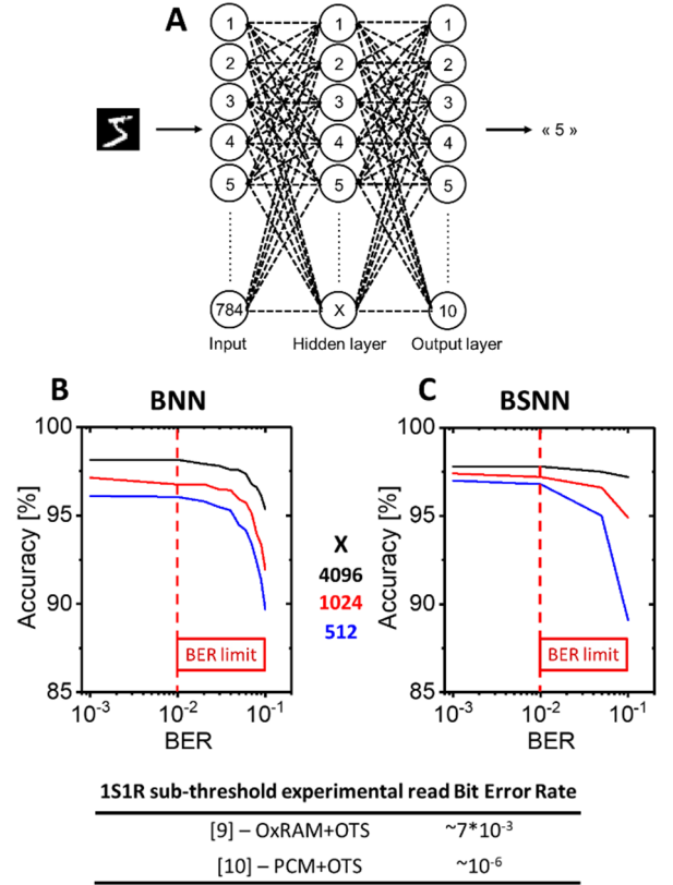
Fig. 7 A) Fully connected neural network topologies with one hidden layer of X neurons are considered in this paper, considering both Binarized Neural Network (BNN) and Binarized Spiking Neural Network (BSNN). The MNIST handwritten digit recognition task is considered. B) (resp. C) ) BNN (resp. BSNN) accuracy evolution with the synaptic binarized Bit Error Rate (BER). No adapted training strategy to the BER is considered in this study. The experimental results provided in [9-10] are demonstrated to be perfectly tolerated by the BNN (resp. BSNN) networks.
