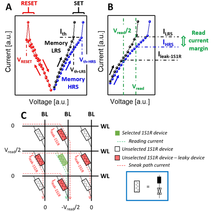
Fig. 2 A) Typical 1S1R quasi-static current-voltage characteristics. The resulting 1S1R switching voltages are strongly influenced by the memory resistive state. If the memory is at the High Resistive State, V_{th-HRS} is required for 1S1R device switching operation. If the memory is at the Low Resistive State, V_{th-LRS} is required for 1S1R device switching operation. B) 1S1R sub-threshold reading operation description, enabling to perform 1S1R read operation while preventing the OTS selector switching. A reading voltage V_{read} , lower than V_{th-LRS} , is required for reading operation. If the memory is at the Low Resistive State, I_{LRS} current is read. If the memory is at the High Resistive State, I_{HRS} current is read. Therefore, the I_{LRS}/I_{HRS} ratio corresponds to the 1S1R sub-threshold read current margin. C) V_{read}/2 1S1R Crossbar array biasing scheme of interest, used to perform the reading operation on an individual 1S1R device in the array. In this biasing configuration, the neighboring 1S1R devices sharing the same Crossbar Word-Line and Bit-Line contribute to the overall leakage current in the array.
