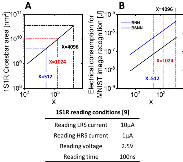
Fig. 8 A) Crossbar footprint evolution with the number of neurons in the hidden layer of the network. The area required for peripherals accommodation is not considered. B) Electrical consumption, associated to 1S1R device read operation, per MNIST image classification evolution with the number of neurons in the hidden layer of the network. The considered reading conditions are provided, based on experimental results published in [9]. Both BNN and BSNN (with 0.13 spikes per neuron per inference) are considered.
