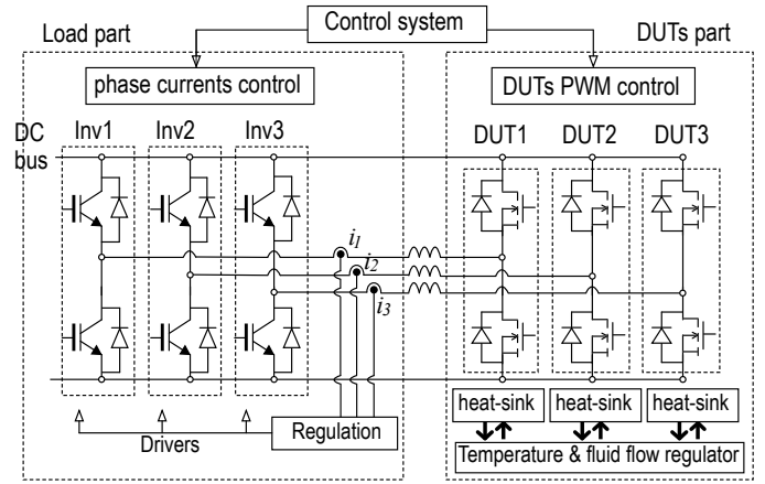
Fig. 2. Switching mode power cycling scheme.
