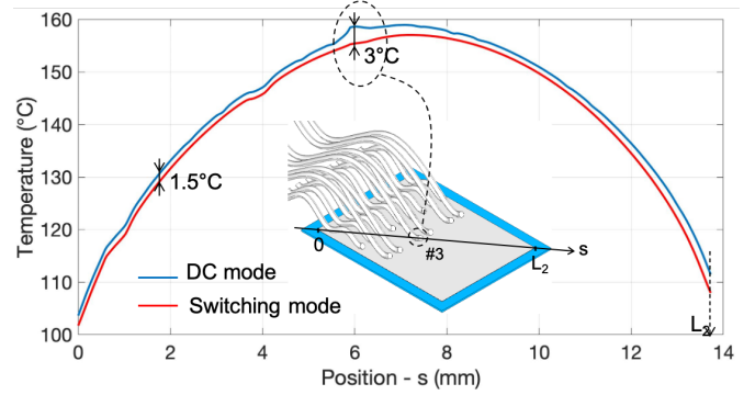
Fig.11. Temperature distribution of the top surface metallization along the diagonal line at t = 3\text{s} .
