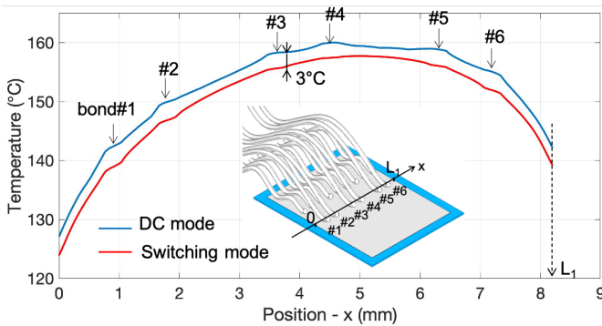
Fig.10. Temperature distribution of the top surface metallization along the transversal line (under the bondwire contacts) at t = 3\text{s} .
