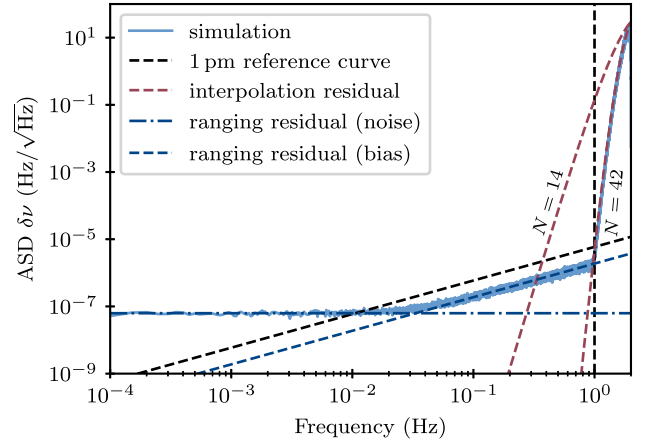
FIG. 8. Processing residuals in application of the fractional delay filter containing ranging errors. We compare the numerically simulated data (solid blue) against the analytical models for the ranging residual caused by ranging noise (dashed-dotted blue) and a constant bias (dashed blue). Additionally, we plot models for the interpolation residual (dashed red) for different interpolation kernel lengths N = 14, 42 alongside the picometer reference curve in dashed black for reference.
