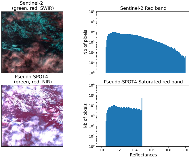
Fig. 4. Above: Sentinel-2 image patch with a histogram of the red band. Below: saturated pseudo-SPOT4 image patch with a histogram of the red band.
