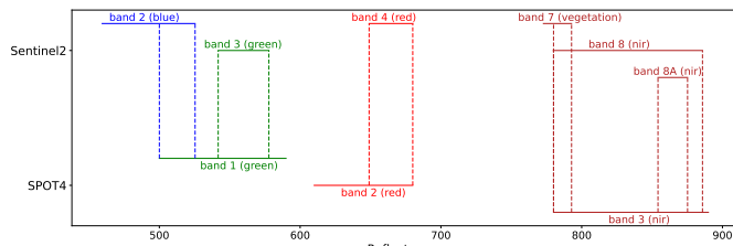
Fig. 2. SPOT4 spectral bands and corresponding Sentinel-2 spectral bands.
