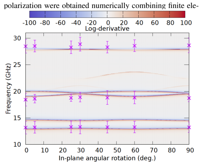
FIG. 3. In-plane dispersion of elastic waves in the thin film Z-LN on Z-Sapphire at a fixed wavenumber k/2\pi = 3.53 \mu\text{m}^{-1} . Angles 0^\circ and 90^\circ correspond to propagation along the x -axis and the y -axis, respectively. Purple crosses are the surface BLS measurements (performed at \theta = 70^\circ ).
