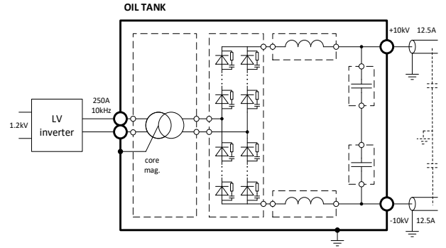
Fig. 3: Schematic of the converter, with entire MV circuit inside of the tank and LV inverter outside of the tank.
