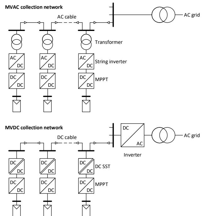
Fig. 1: PV MVAC versus MVDC power collection network diagram.
