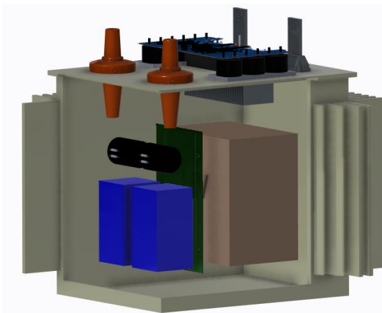
Fig. 2: DC-SST mechanical arrangement with MFT (brown), rectifier (green), inductors (blue) and capacitors (black) immersed in the oil tank and low voltage inverter sitting on top of the tank.
