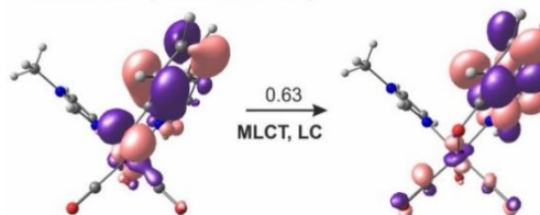
Transition 8: (311 nm, 5.2 \cdot 10^{-2} )
