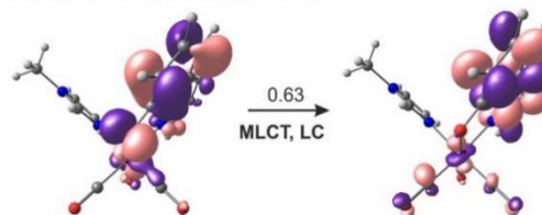
Figure 8 Natural transition orbitals for the first and main transitions of 2 in the 310-480 nm region. The excitation energy and the corresponding oscillator strengths are indicated in parentheses and the associated weights above the arrows (isodensity surface 0.043). For each transition, only the component associated to the highest weight is displayed and the main excited state character is indicated under the arrow (MLCT stands for metal-to-ligand-charge-transfer, MC for metal-centered and LC for ligand-centered charge transfer).
