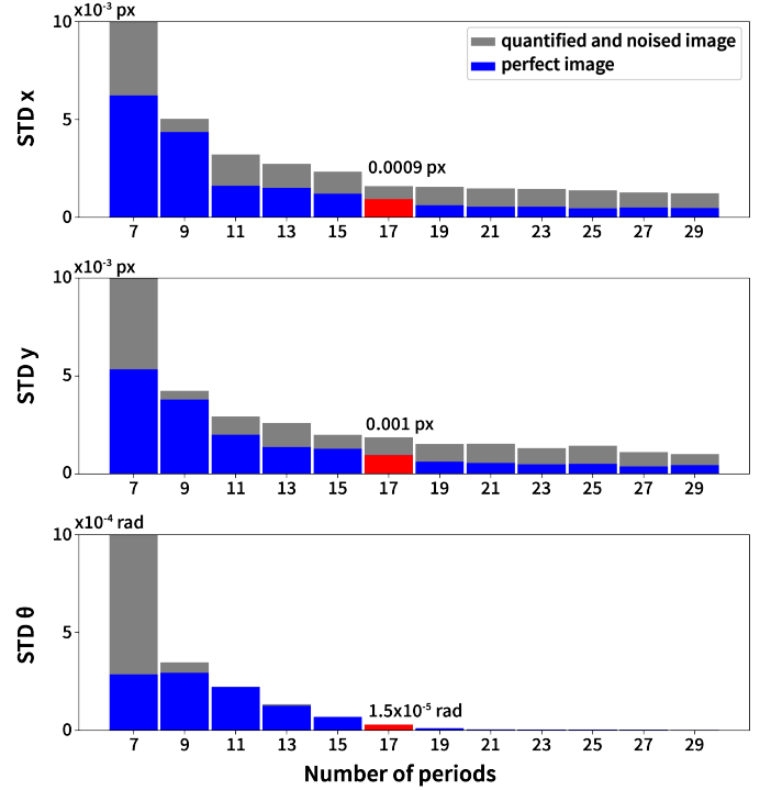
Fig. 4. Evolution of the standard deviation of the position and orientation errors computed on 100 frames for different numbers of periods contained in the HP code. Both perfect and noised images are simulated and highlighted respectively in blue and gray.
