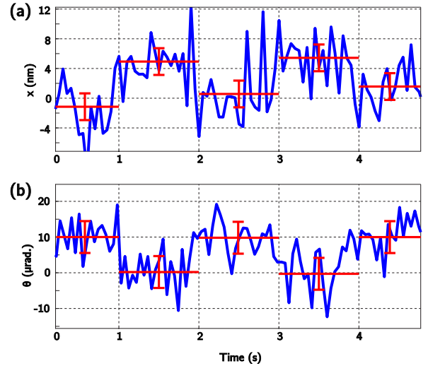
Fig. 6. Resolution tests with 5 nm height squares input signal for the translation and 10 \mu rad for the rotation. Horizontal red lines represent the mean value of each step (20 images each) and vertical bars represent the standard deviation of the static noise studied in Section III-B2.
