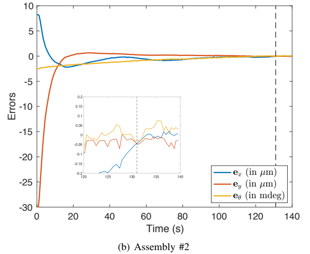
Fig. 10. Evolution of the position and orientation errors during visual servoing after coarse positioning (as in Fig. 10.(a)) for two chip assemblies.
