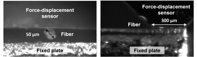
Fig. 13. Polyamide 11 fiber during compression tests along: cross section (left), length (right).
