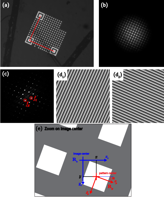
Fig. 3. Major steps of the phase-based position measurement: (a) HP code as acquired by the camera; (b) sub-image taken at the center of the HP code with a Hanning window; (c) Fourier spectrum exhibiting the two peaks f_1 and f_2 ; ( d_1 ) and ( d_2 ) show the inverse Fourier transform after bandpass filtering of each of the peaks; and (e) highlights the shift presented in Eq. 3 between the rough center of the HP code and the phase-based center.
