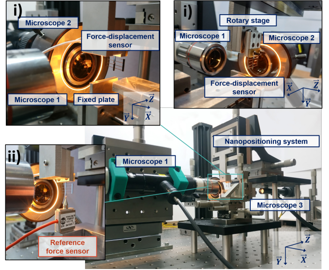
Fig. 12. Experimental setup in: (i) fiber characterization configuration, (ii) sensor calibration configuration.
