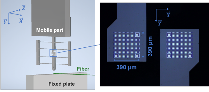
Fig. 11. Force-displacement sensor made of a CT joint compliant structure and including two HP codes.
