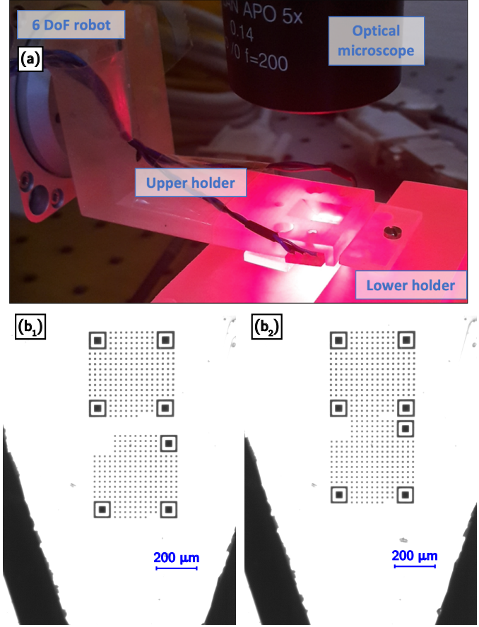
Fig. 8. Experimental setup for the assembly of microfluidic chips. (a) Close view of the experimental setup. (b 1 ) and (b 2 ) Images of the HP codes before and after the visual servoing. The left HP code is part of the lower plate of the fluidic chip, while the right HP code is part of the upper one.
