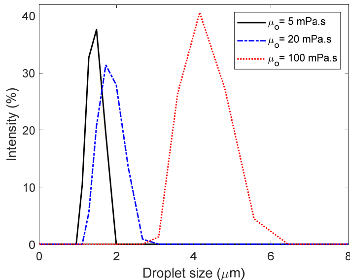
Figure 2: Droplet size distribution of the inner aqueous droplets ( \mu_{wi} = 1 \text{ mPa s} ) with varying viscosity of the oil phase.
