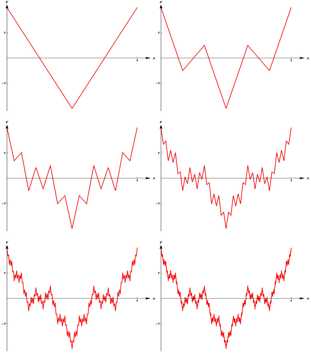
Figure 2: The prefactal graphs \Gamma_{\mathcal{W}_0}, \Gamma_{\mathcal{W}_1}, \Gamma_{\mathcal{W}_2}, \Gamma_{\mathcal{W}_3}, \Gamma_{\mathcal{W}_4}, \Gamma_{\mathcal{W}_5} , in the case when \lambda = \frac{1}{2} and N_b = 3 . For example, \Gamma_{\mathcal{W}_1} is on the right side of the top row, while \Gamma_{\mathcal{W}_4} is on the left side of the bottom row.
