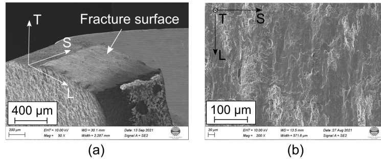
Figure 1: The flat fracture surface of aluminum alloy 2198-T8R under shear loading adapted after Kong et al. [2023a].
