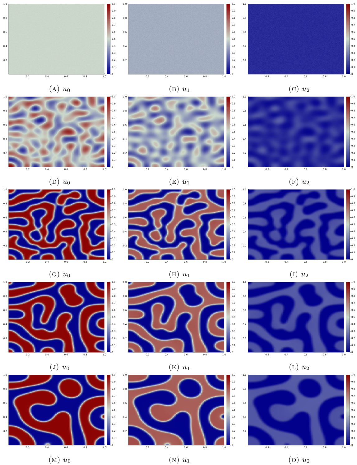
FIGURE 5. Spinodal decomposition successively at times t = 0, 0.06, 0.13, 0.49, 1.5 .
