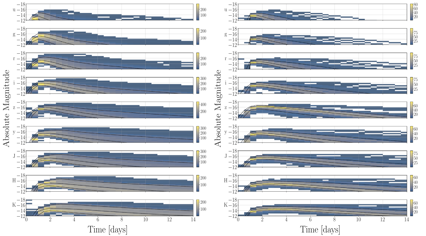
Figure 7. 2D histograms of simulated BNS (left) and NSBH (right) light curves for O4. We show light curves in u , g , r , i , z , y , J , H bands in order to include all the bands used by surveys considered in this work (ZTF, Rubin, and Gemini). In each panel, we plot three dash lines; on top the 10th percentile, at middle the 50th percentile and on bottom the 90th percentile. The color bar shows the number of detections in the different bands. For the observing run O5, see Figure 16, in Appendix B.1.
