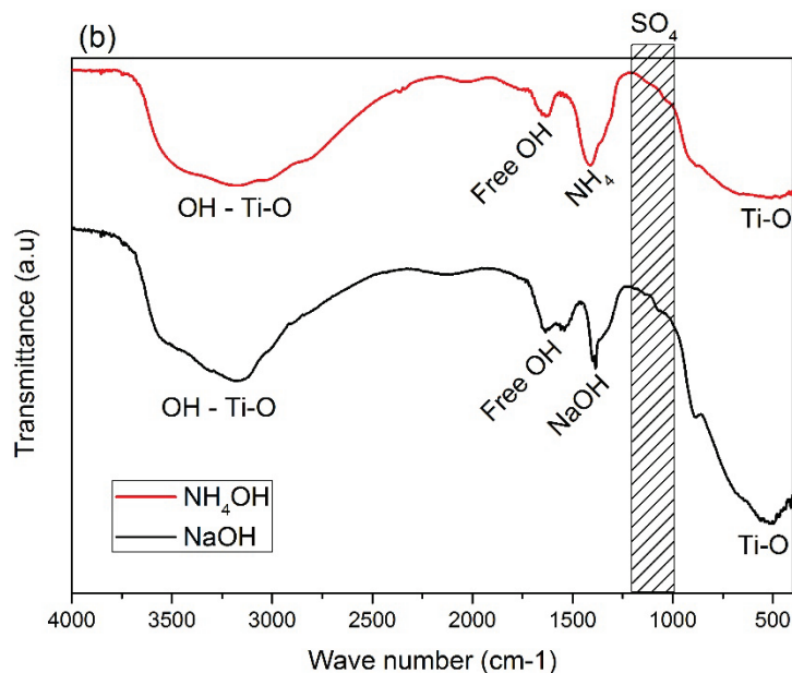
Figure 1: (a) XRD patterns obtained on \text{TiO}(\text{OH})_2 precursor synthesized by ammonium hydroxide and sodium hydroxide routes. (b) corresponding FTIR data.
