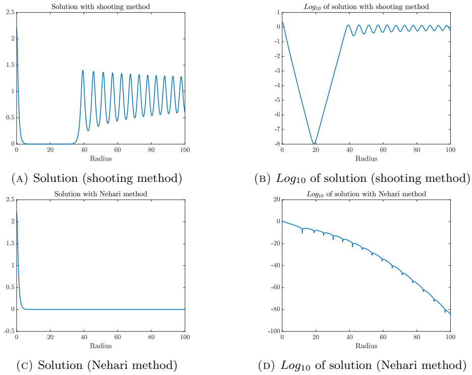
FIGURE 2. Computation of a ground state on large domain
