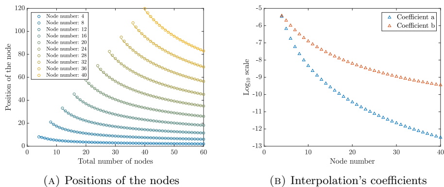
FIGURE 8. Nodes positions and interpolation by k \mapsto 1/\sqrt{ak + b}
