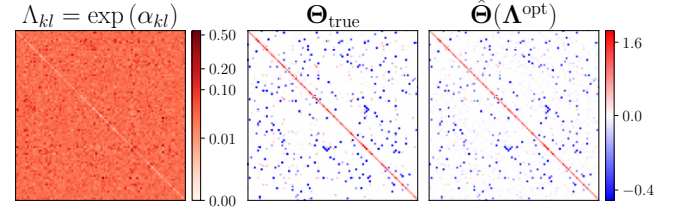
Figure 3 – Visualization of the matrices \Lambda^{\text{opt}} , \Theta_{\text{true}} and \hat{\Theta}(\Lambda^{\text{opt}}) .
