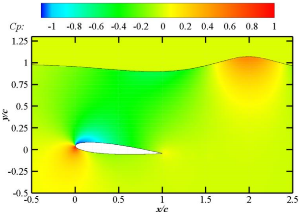
(B) h/c = 1.03
