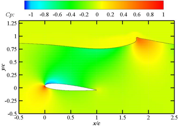
(C) h/c = 0.91
