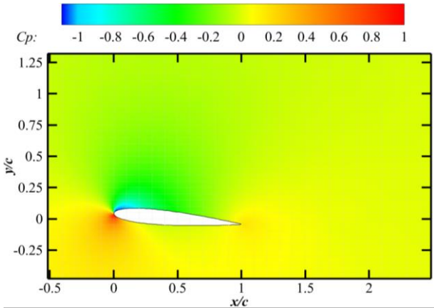
(A) h/c = 4.0
