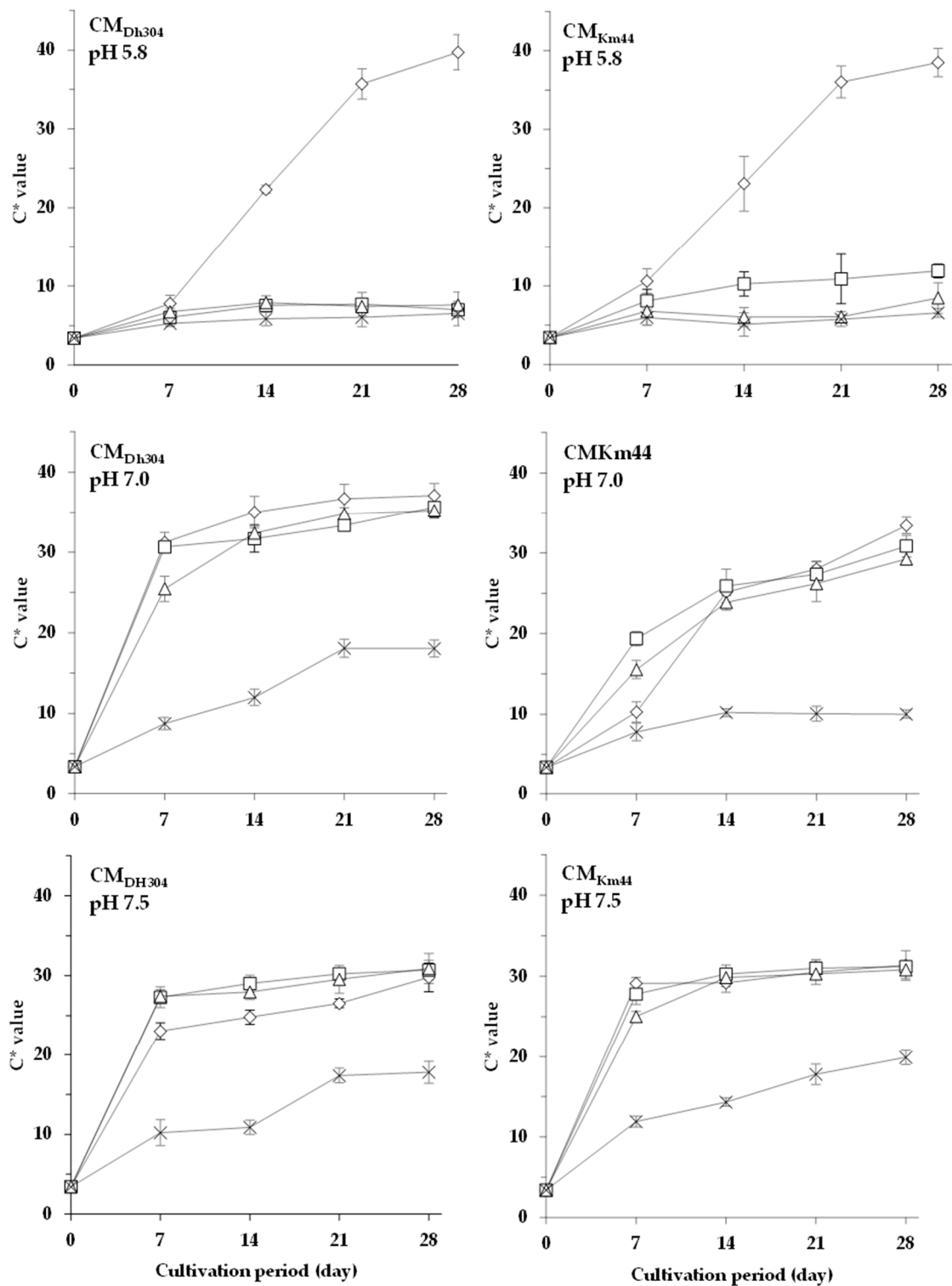
Figure 4. Changes in saturation C* of Arthrobacter arilaitensis Po102 cultures during cultivation on CM Dh304 and CM Km44 at the initial pH 5.8, 7.0, and 7.5. Culture conditions in various amounts of NaCl: 0% (—◇—), 2% (—□—), 4% (—△—), and 8% (—×—).
