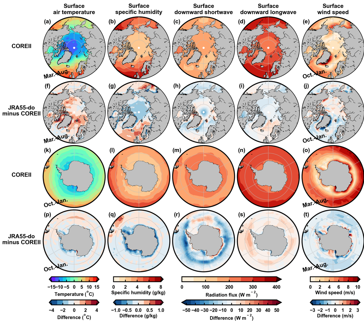
Figure 6. 1980–2007 March–August mean Arctic and October–January mean Antarctic surface air temperature (first column) and specific humidity (second column), downward shortwave (third column) and longwave radiation (fourth column) fluxes, and October–January mean Arctic and March–August mean Antarctic surface wind speeds (fifth column). The first and third rows correspond to CORE-II, and the second and fourth rows are differences between JRA55-do and CORE-II.
