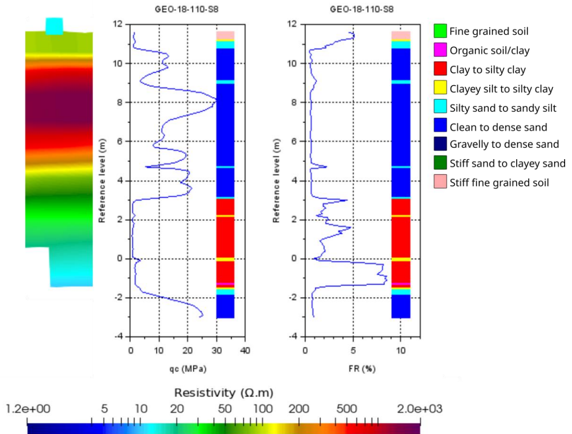
Figure 41 : Resistivity of ERT_L2_S6 profile compared with q_c and R_f at CPT S8
