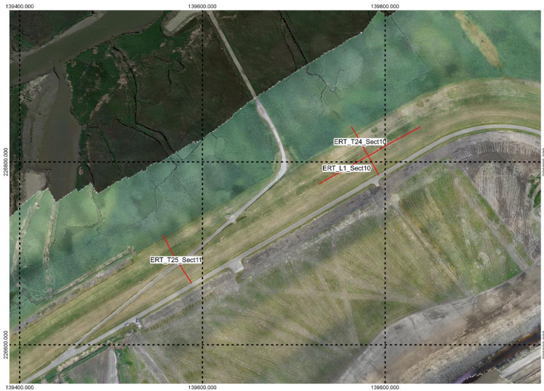
Figure 5: ERT profiles location of sections 10 and 11
