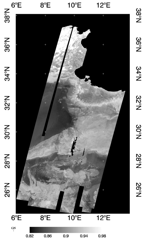
Figure 3. Window emissivity created using ASTER thermal data of 400 x 1200 km region in a part of Sahara Desert.
