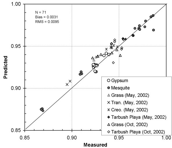
Figure 1. Measured window emissivities by CIMEL CE312 and predicted values using linear regression. Measurements were made in Jornada Experimental Range and in White Sands National Monument, New Mexico, USA.
