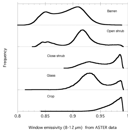
Figure 4. Histograms of window emissivities for each land cover type in the study area. The values of Barren and Open shrub range widely between 0.82 to 0.96.
