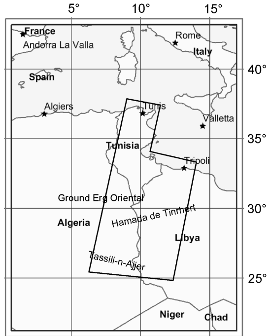
Figure 2. The study area over Tunisia, Algeria, and Libya. 258 scenes of ASTER data are used to cover this area.
