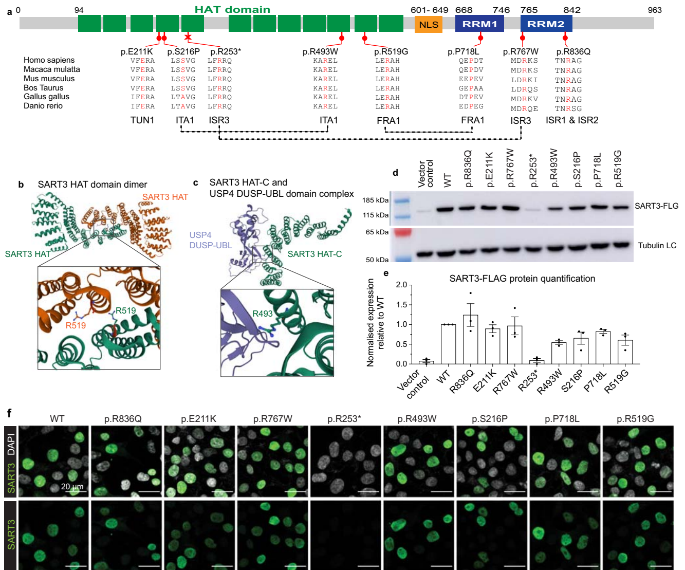
Fig. 2 | SART3 variants map to conserved domains and residues. a SART3 is a 963 amino acid protein containing 12 half-a-tetratricopeptide (HAT) repeats (the HAT domain, green), a nuclear localisation signal (NLS, yellow) and two RNA recognition motifs (RRM1 and RRM2, blue). Positions of SART3 variants are shown in red. Variants show amino acid conservation between vertebrate species. b Crystal structure of human SART3 HAT domains as a dimer (PDB ID 5CTQ) with Arginine 519 highlighted on each chain. c Crystal structure of human SART3 HAT-C domain-human USP4 DUSP-UBL domain complex (PDB ID 5CTR) with Arginine 493 highlighted. Crystal structures were visualised in the RCSB PDB 3D protein viewer (Mol*). d Western blot analysis of WT and variant pCMV-SART3-FLAG constructs transiently transfected in HEK293t cells with an anti-FLAG antibody and beta-
