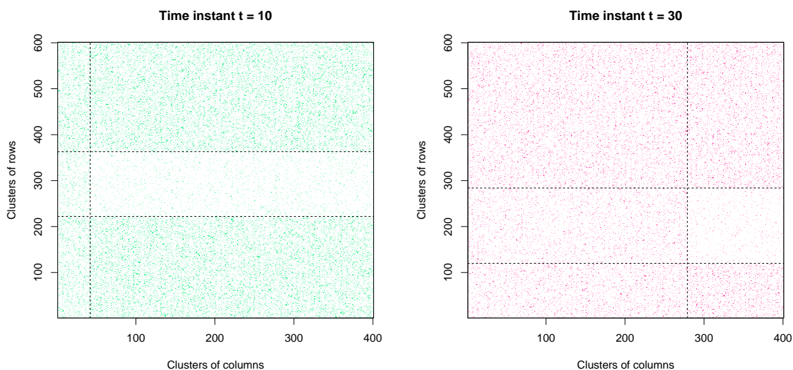
Figure 3: Reorganized incidence matrices at time instants t = 10 and t = 30 according to the estimates of the cluster memberships. Nearby rows (columns) belong to the same cluster of rows (columns). The blocks are also delimited by black dashed lines.
