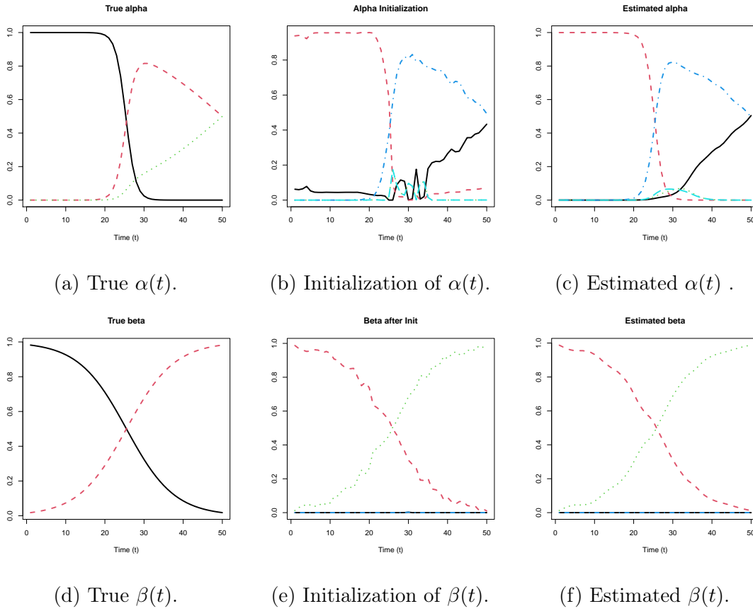
Figure 5: Evolution of the true (left), initialized (center) and estimated (right) proportions of the parameters \alpha(t) and \beta(t) , respectively.
