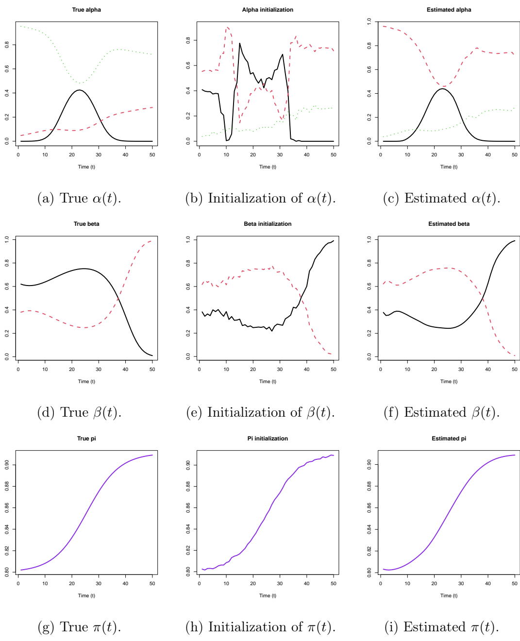
Figure 6: Evolution of the true (left), initialized (center) and estimated (right) proportions of the parameters \alpha(t) , \beta(t) and \pi(t) , respectively.
