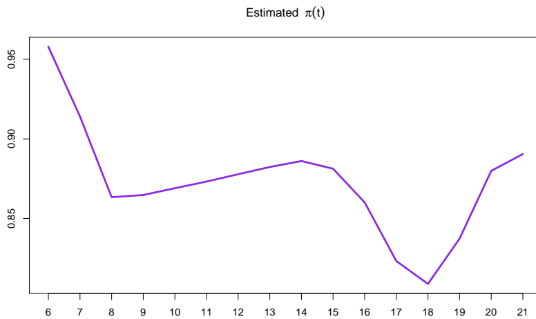
Figure 10: Evolution of \hat{\pi}(t) estimation.
