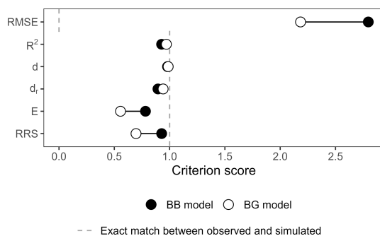
Figure A1. Score of the BB and BG transformations according to other common and recently developed performance criteria: the root mean square error (RMSE), the coefficient of determination R^2 , the index of agreement d (Willmott, 1981), the refined index of agreement d_r (Willmott et al., 2012), the Onyutha efficiency E , and the revised R^2 (RRS) (Onyutha, 2022).
