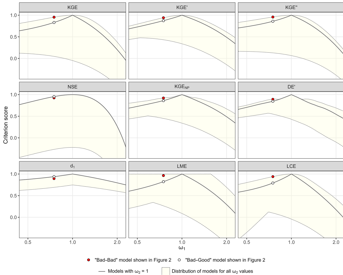
Figure 4. Score of each transformation for all [ω 1 ; ω 2 ] combinations by performance criteria.
