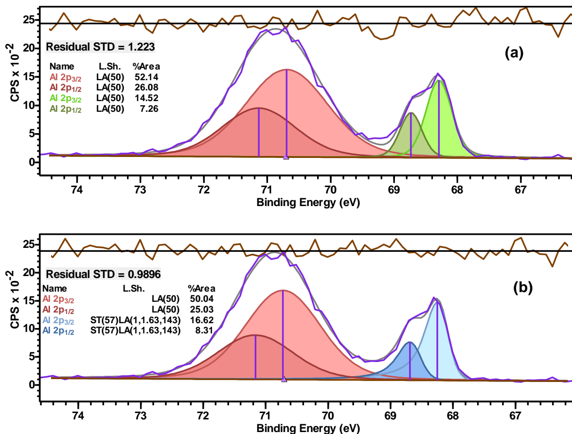
Figure 63. Peak fitting of the metallic signal in the Al 2p peak envelope with (a) symmetric LA line shapes (Voigt functions) and (b) asymmetric LA line shapes with a parameter (ST) that controls the exponential tail. Both the ST parameter and the second LA parameter/peak shape with a value of 1.63 in the LA function control the exponential tail (asymmetry).
