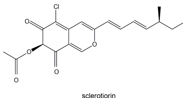
Figure 5. Chemical structure of the pigment sclerotiorin produced by Penicillium sclerotiorum 2AV2.
