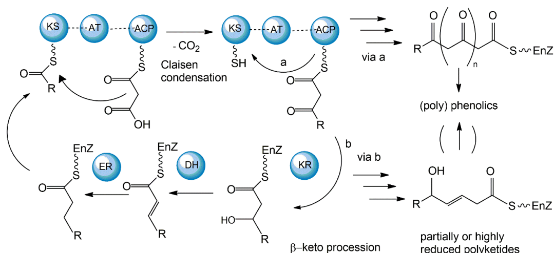
Figure 6. Mechanisms of fungal polyketide biosynthesis.
