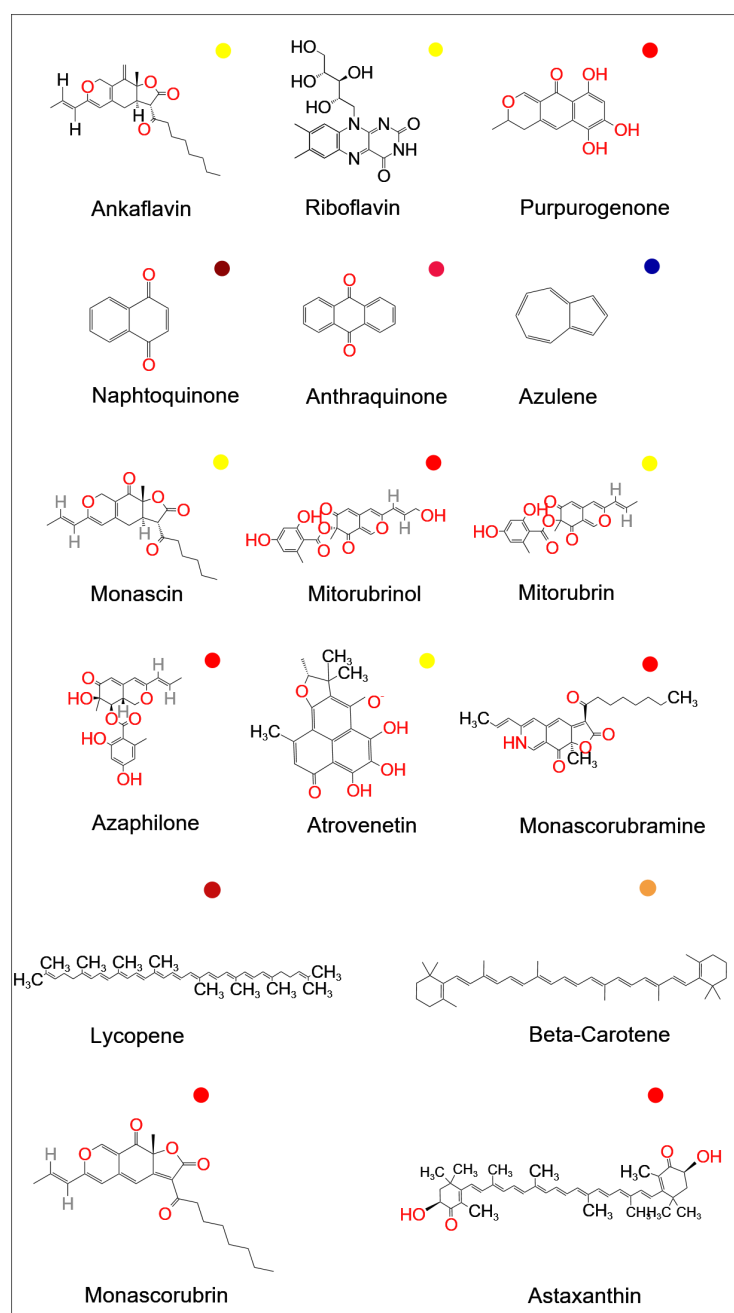
Figure 4. Chemical structure of some available fungal food pigments (Source: National Center for Biotechnology Information. PubChem Compound Database; ( https://pubchem.ncbi.nlm.nih.gov ); accessed on 1 April 2023).
