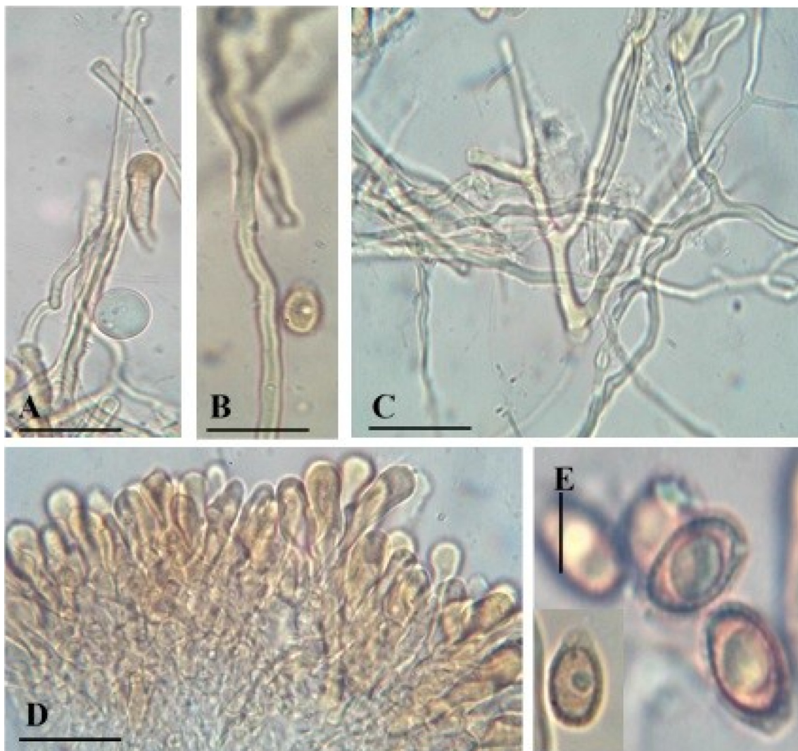
Fig. 3. Microscopic structures of Ganoderma multistipitatum (A–E GCB101). A–C. Hyphae (A. Generative), (B. Skeletal), (C. Binding). D. Cells of crustohymeniderm. E. Basidiospores. Bars = 5 \mu\text{m} (A–C), 10 \mu\text{m} (D–E).
