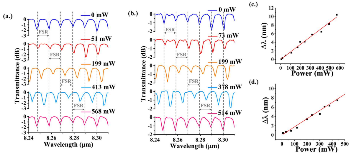
Fig.4. Measured transmission spectra of a racetrack resonator (radius 250 \mu\text{m} , coupling length 45 \mu\text{m} ) for different power dissipated in the heater of different gaps of; (a.) 0.8 \mu\text{m} and (b.) 1.0 \mu\text{m} ; the gray lines indicate the FSR of the device. Resonance shifts around 8 \mu\text{m} wavelength as a function of the power dissipated in the heater of racetrack with 250 \mu\text{m} radius, 45 \mu\text{m} coupling length and the gap of (c.) 0.8 \mu\text{m} and (d.) 1.0 \mu\text{m} ; solid red line indicated the linear fitting used to estimate the thermal heating performance.
