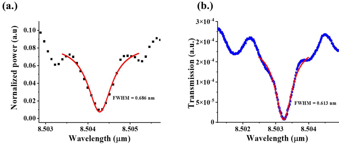
Fig.5. Confirmation of the calibration procedure. Transmission of a resonator (radius 250 \mu\text{m} , coupling length 30 \mu\text{m} ) when measured (a) using the DFB-QCL laser; (b) using the CW laser and thermal variation inside the resonator.
