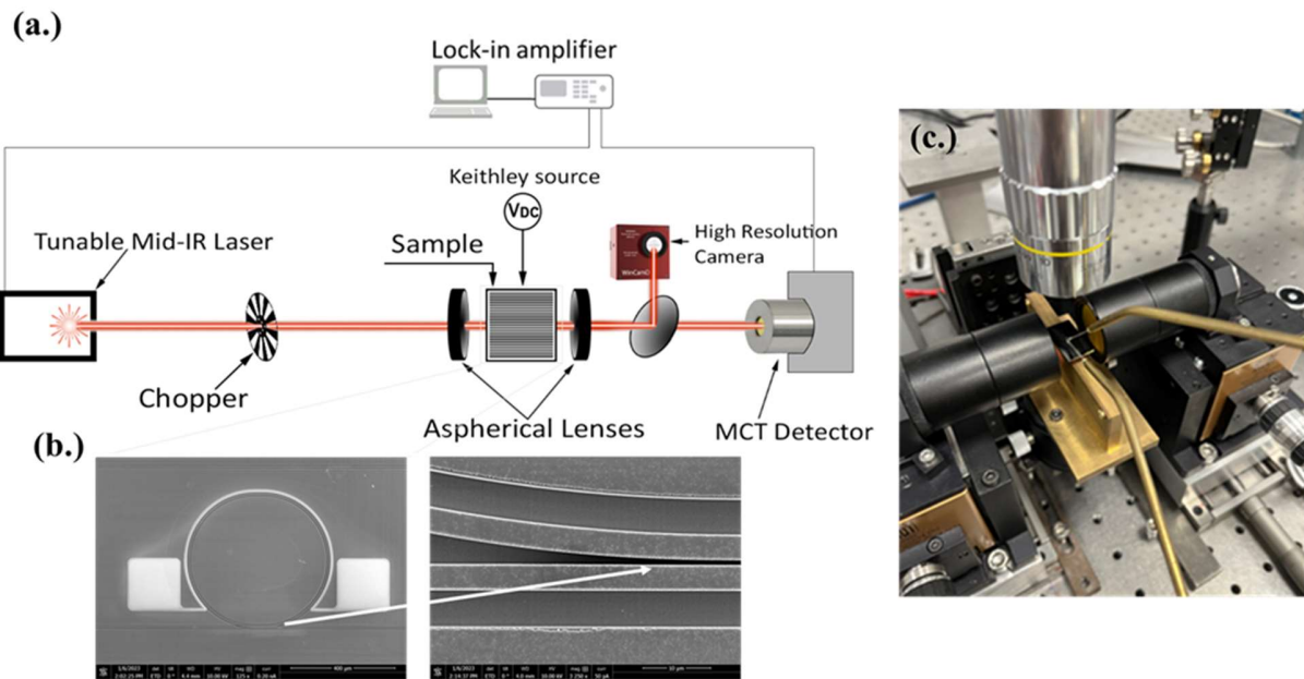
Fig.2. (a.) Schematic view of the experimental setup. (b.) SEM images of the device after fabrication of the racetrack, with zoom-in view on the directional coupler part. (c.) Picture of the device during the measurement.
